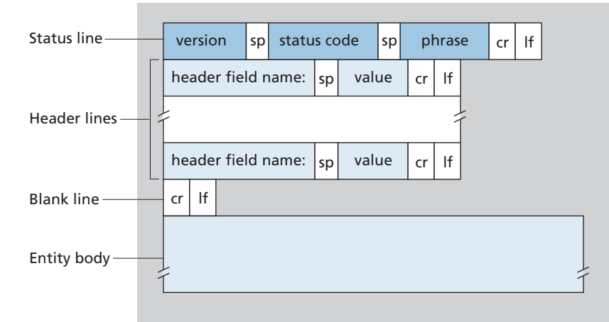
Figure 2.9 ♦ General format of an HTTP response message
